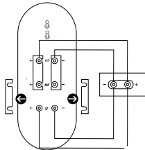
Bi-wiring
