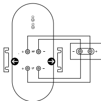
Bi-wiring
